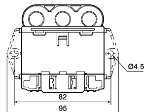
MOUNTINGHOLESIZE
