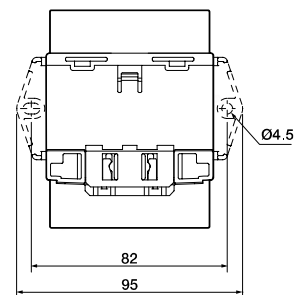
MOUNTINGHOLESIZE
