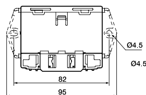
MOUNTINGHOLESIZE
