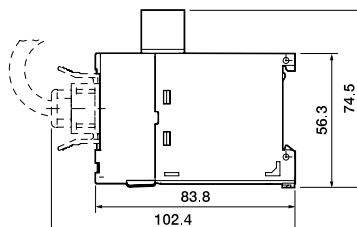
PANEL&DINRAILTYPE
