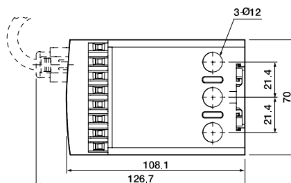
PANEL&DINRAILTYPE
